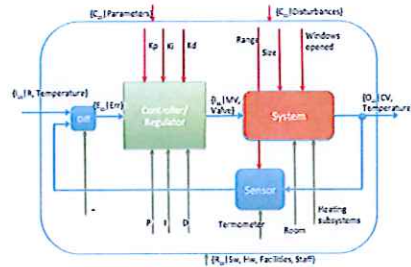
Fig. 2 - A Controlled System
