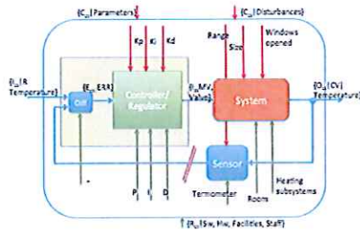
Fig. 3 - Closed and Open loop Control
