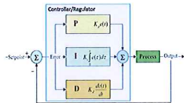
Fig. 4 - The PID Controller
